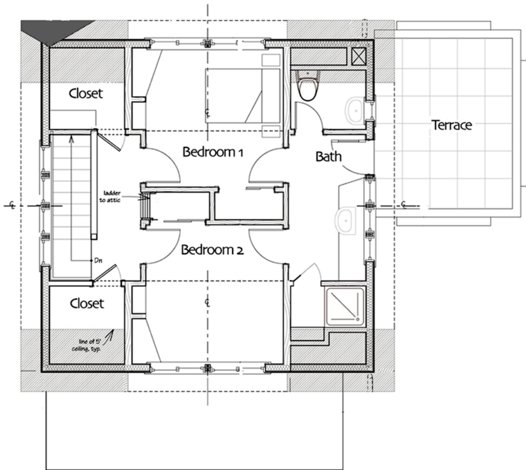
Songbird Optional Second Floor Plan
